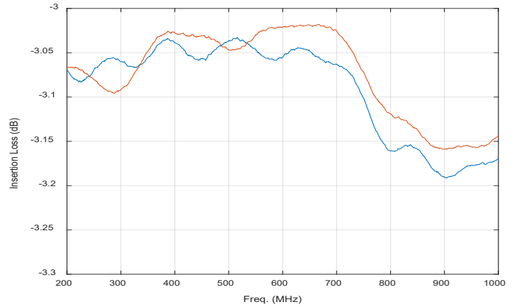
Typical Insertion/Return Loss
