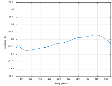
Typical Coupling & Directivity
